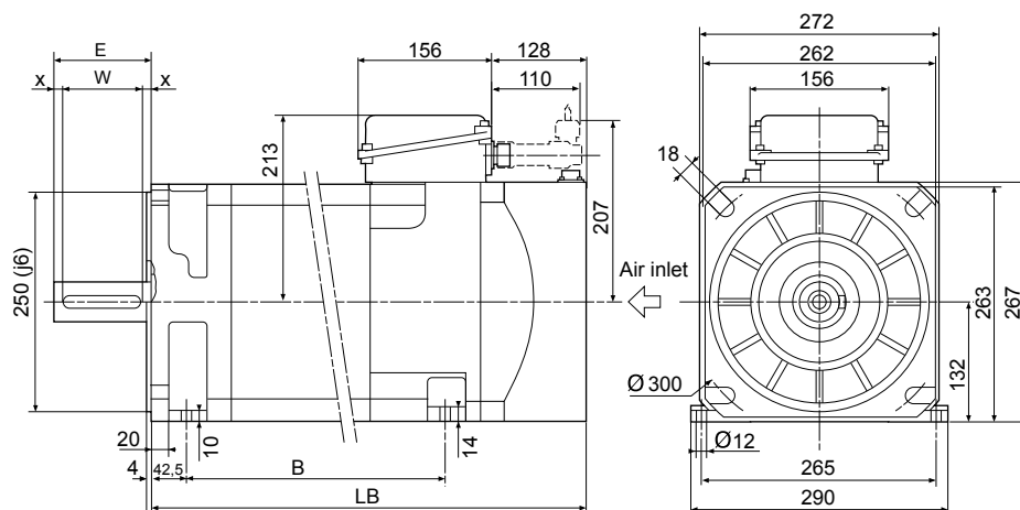
AMS 132 Motor
