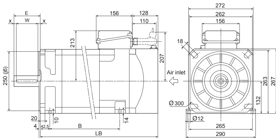
AMS 132 Motor
