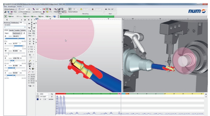
Example of a NUMROTO 3D simulation.
