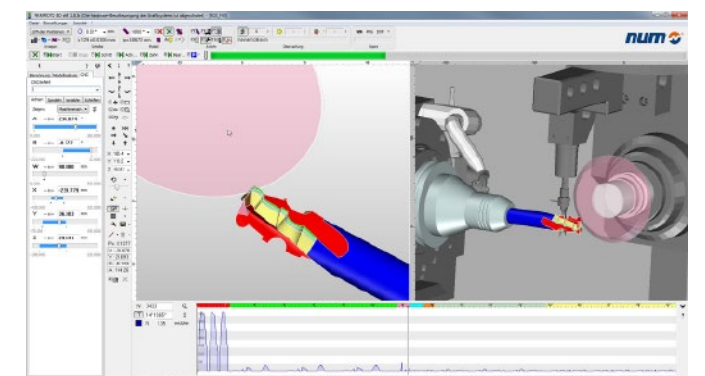
Example of a NUMROTO 3D simulation.
